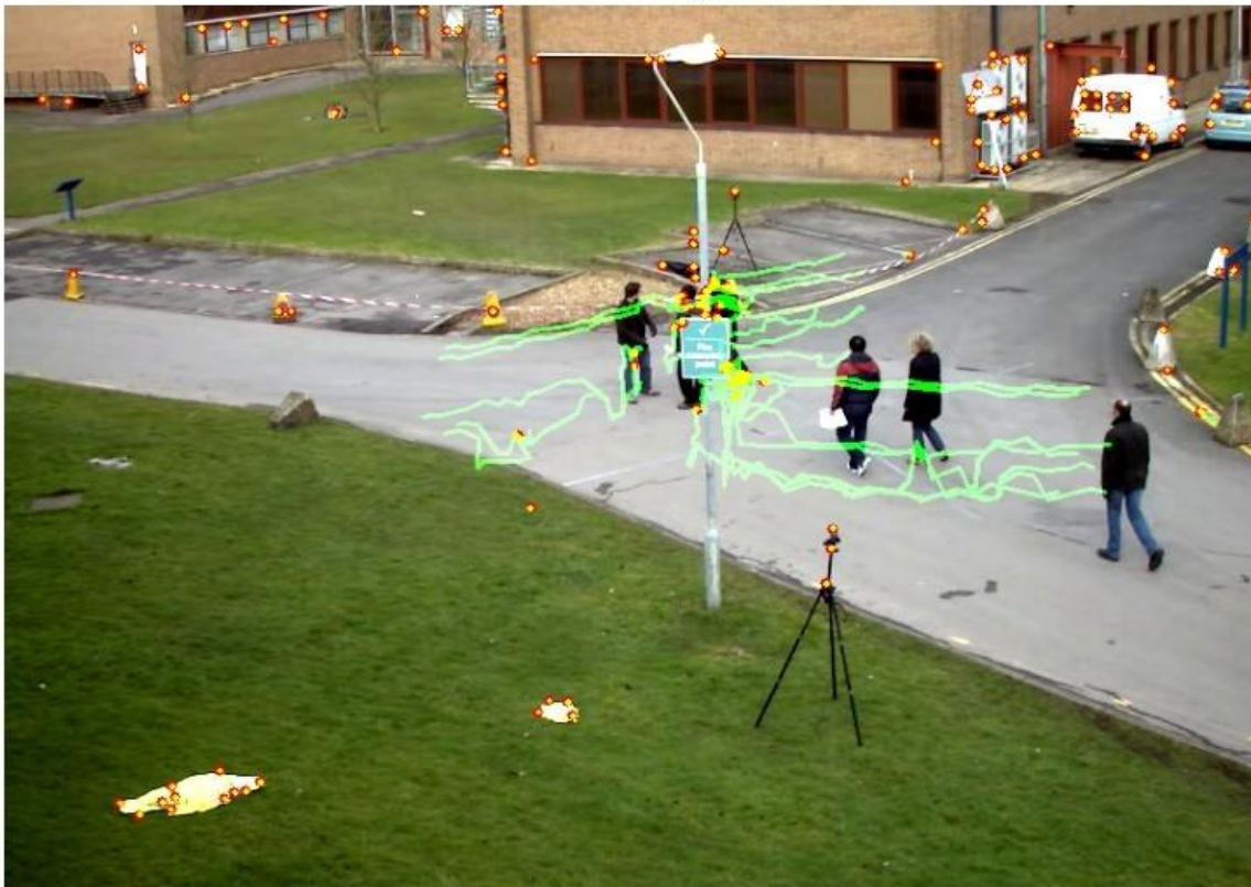
Lucas-Kanade Tracking — Frame 50
